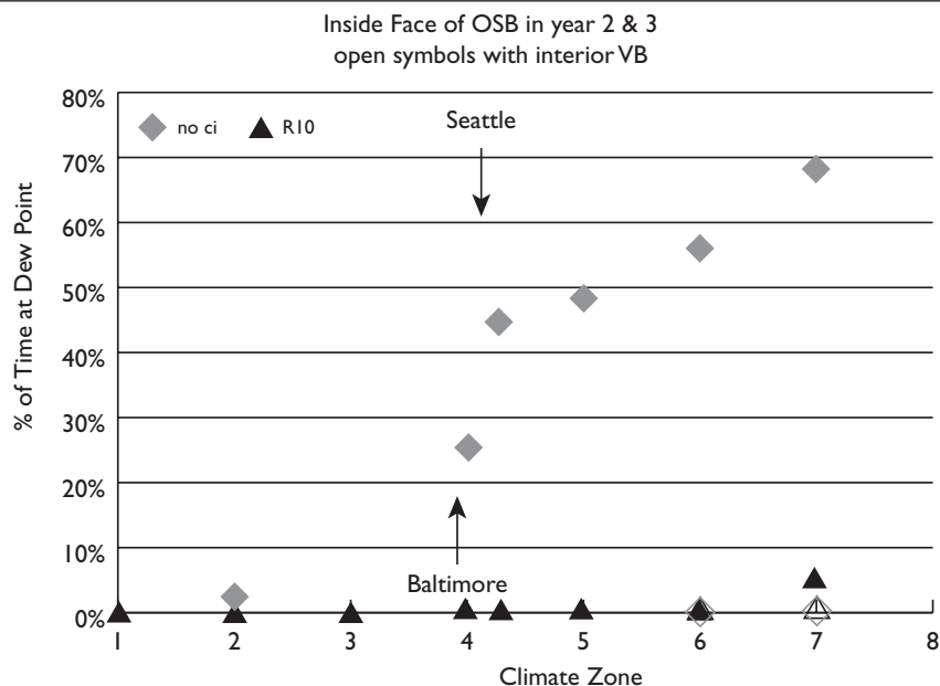
Figure 9 R-10 Sheathing, Influence on Dew Point Occurrence 9
