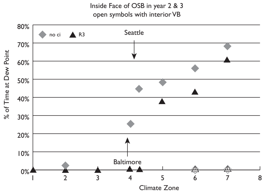
Figure 8 R-3 Sheathing, Influence on Dew Point Occurrence 9
